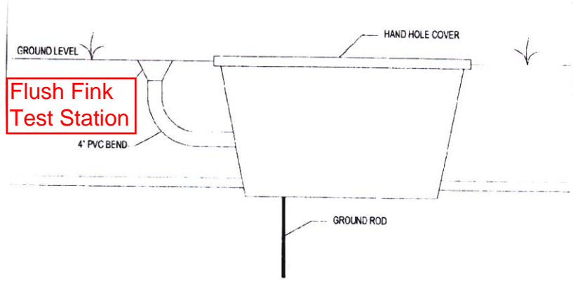
HAND HOLE WITH STREET FINK ELEVATION DETAIL
